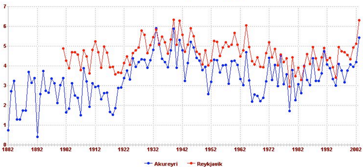
Figure 13 Temperature records for Reykjavik and Akureyri, Iceland
