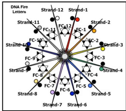
Figure 6. Hebrew Alphabet / DNA Fire Letters
