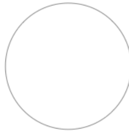
The Original Source Particle (SP)
