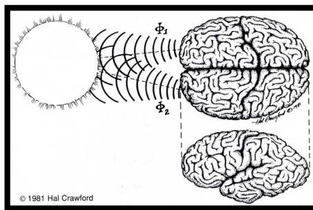
Figure 3. The Human Brain-Scalar Interferometer
