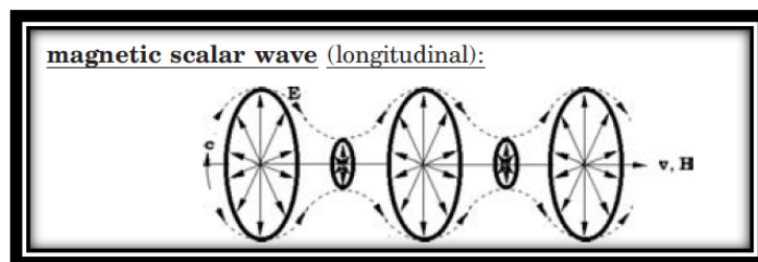
Figure 1. Electric ring vortices form a magnetic wave.
