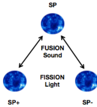
Figure 2. The Perpetual Fission-Fusion Scalar Wave
