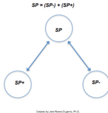
Figure 5. The Source Particle Phasing Process
