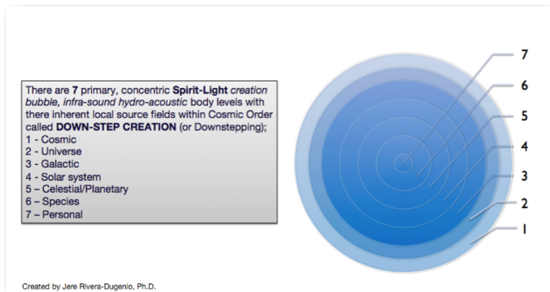
Figure 8. The 7 Concentric, Spirit-Light Creation Spheres
