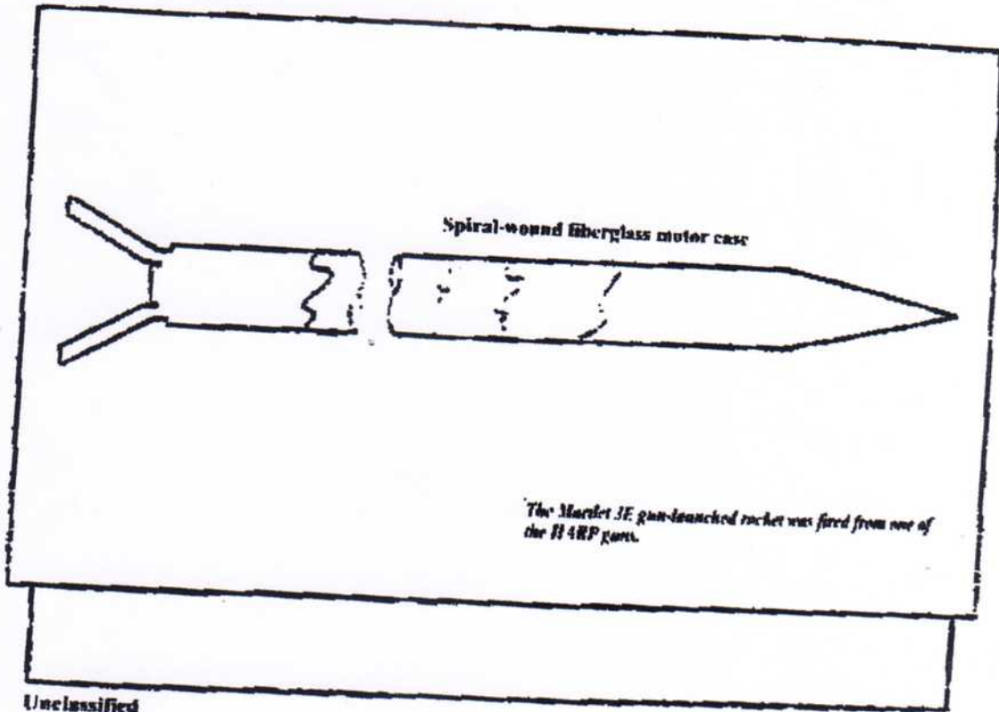
Figure 4 Martlet 3E Gun-Launched Rocket
